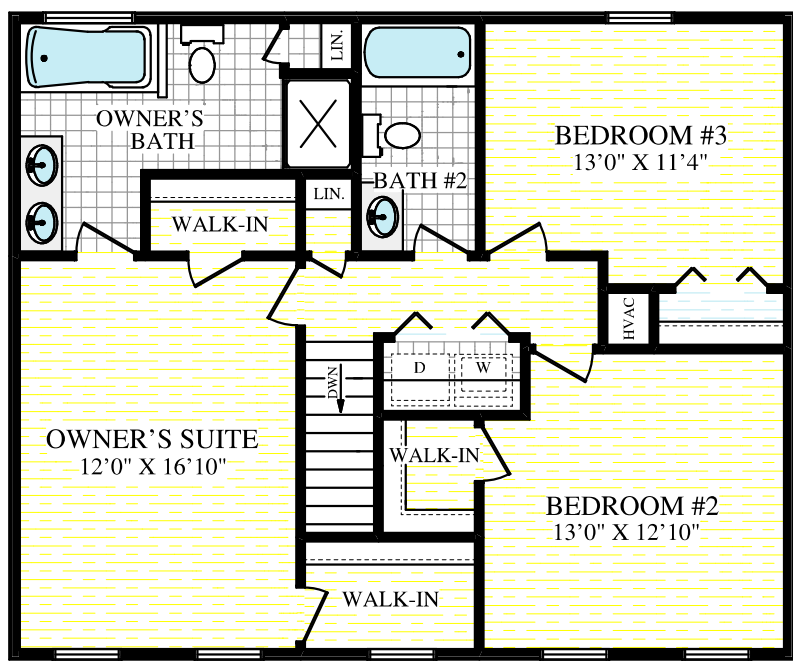
2ND FLOOR LEVEL
